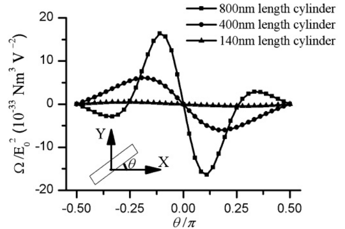
FIG. 6. Optical torques on three kinds of cylinders. For the 140-nm-length cylinder, we have not observed stable equilibrium orientations. For the 400-nm-length cylinder, \theta = 0 is the stable equilibrium orientation. For the 800-nm-length cylinder, in addition to the stable equilibrium orientation at \theta = 0 , metastable orientation is observed at \theta = \pm 0.5\pi .
