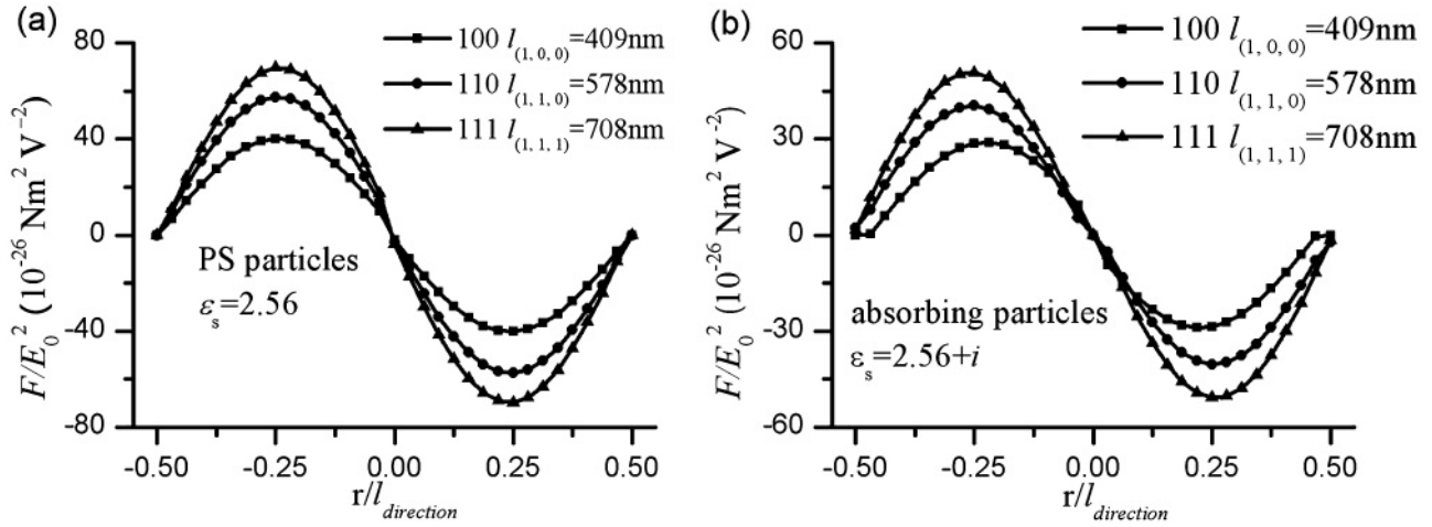
FIG. 5. (a) Optical forces on polystyrene particles arising from the 3D-optical lattice. The shapes of the optical-force lines along different directions are similar. The amplitudes of the optical forces fulfill F_{\max[1,0,0]} = F_{\max[1,1,0]}/\sqrt{2} = F_{\max[1,1,1]}/\sqrt{3} . (b) Optical forces on absorbing particles arising from the 3D-optical lattice.
