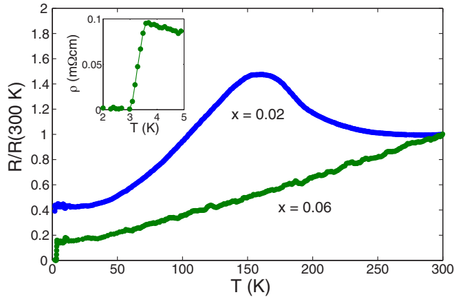
FIG. 1. (Color online) Residual resistance ratio versus temperature for x = 0.02 (blue curve) and x = 0.06 (green curve) samples. The inset shows the superconducting transition with T_c = 3 K for the x = 0.06 sample. The hump at roughly 150 K in the x = 0.02 sample is a signature of the CDW.
