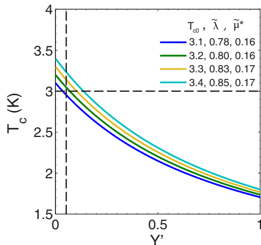
FIG. 4. (Color online) Calculated T_c as a function of the disorder parameter Y' for different values of \tilde{\mu}^* and \tilde{\lambda} . From the intersection of the measured T_c and Y' for x \approx 0.06 , T_{c0} where Y' = 0 can be backtracked.
