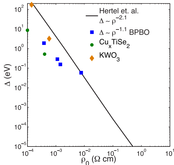
FIG. 3. (Color online) Correlation gap as a function of the zero-temperature resistivity for \text{Nb}_x\text{Si}_{1-x} (black line), \text{BaPb}_{1-x}\text{Bi}_x\text{O}_3 (blue squares), \text{K}_{0.33}\text{WO}_3 thin films with different thicknesses (orange diamonds), and \text{Cu}_x\text{TiSe}_2 (green circles) for Cu concentration x = 0.02 and 0.06 .
