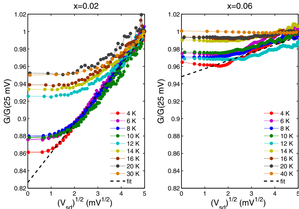
FIG. 2. (Color online) Normalized differential conductance G versus the square root of the source drain voltage V_{sd} in units of (\text{mV})^{1/2} for \text{Cu}_x\text{TiSe}_2 with (a) x = 0.02 and (b) x = 0.06 . The black dashed lines are fits used to extract the normalized zero-temperature DOS and correlation gap.
