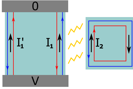
FIG. 1 (color online). Using helical quantum edge gears to measure the Luttinger parameter. We consider \mathbb{Z}_2 TI edge states in two adjacent topological regions. The blue and red arrows indicate the propagation directions of edge electrons with opposite helicities. The left TI is connected to external leads; I_1 and I_1' denote the currents of the edges connected to these. The right TI edge floats as an electrically isolated closed loop. Rashba spin-orbit coupling [1] enables Coulomb drag due to short-ranged spin-flip scattering [23] between the adjacent edges. This induces a current I_2 that circulates in the right edge. In the case of identical TIs with an interacting edge region of size L \rightarrow \infty , at zero temperature strong backscattering “locks” the currents I_1 = I_2 , associated to perfect drag [10,12]. We then predict that the zero-temperature conductance is G = (I_1 + I_1')/V = (e^2/h)(2K + 1)/(K + 1) , where K is the Luttinger parameter. In a real system of finite length L \gg \xi and at temperatures T satisfying \hbar v/L \lesssim k_B T \ll \Delta [11] with \xi = \hbar v/\Delta and \Delta the Mott gap of the antisymmetric mode, the result for G holds up to terms exponentially small in L/\xi and \Delta/k_B T [10–12]. Here v is the charge velocity.
