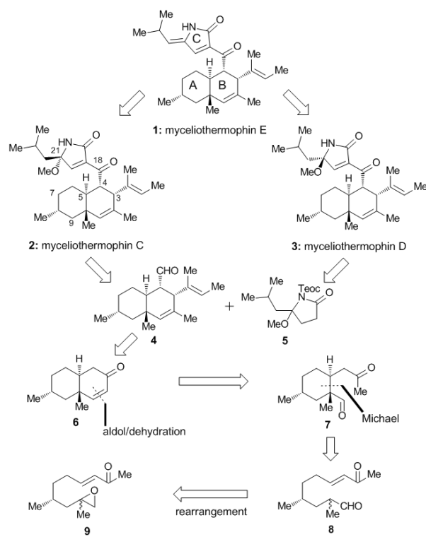
Figure 1. Structures of myceliothermorphins E ( 1 ), C ( 2 ), D ( 3 ) and retrosynthetic analysis.
