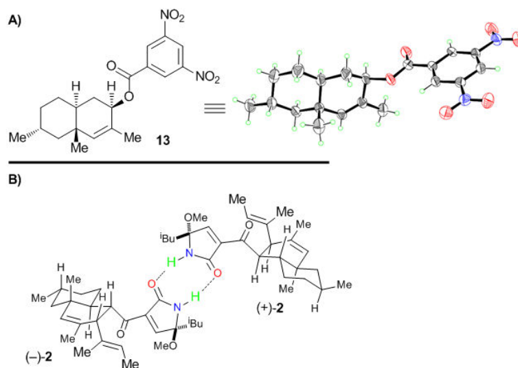
Figure 2. X-Ray derived ORTEP representation of A ) 3,5-dinitrobenzoate ( \pm )- 13 and B ) synthetic myceliothermophin C [ \pm ]- 2 . Thermal ellipsoids at 30% probability. gray = C, red = O, blue = N, green = H for both ORTEPS.
