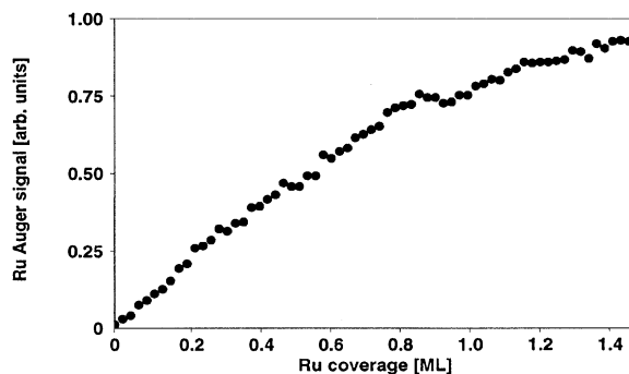
FIG. 1. Auger peak-to-peak height of the Ru 231 eV line versus Ru coverage on C(0001). The coverage is referred to the atomic density of the bulk Ru(0001) plane. Statistical errors are contained within the symbol size.
