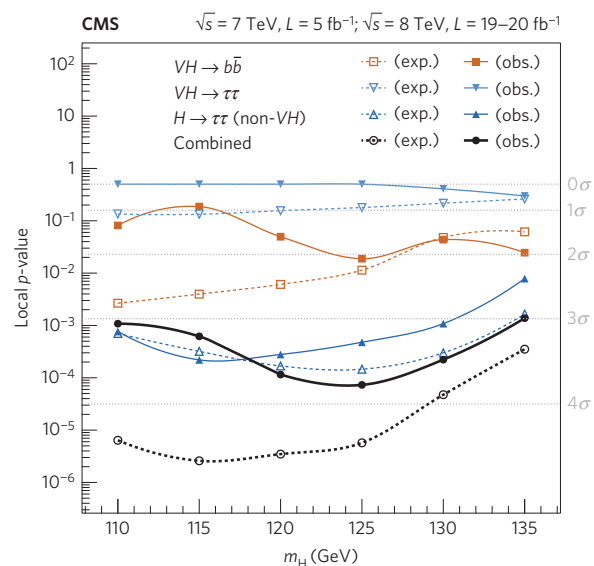
Figure 1 | The p -value for the background-only hypothesis as a function of the Higgs boson mass hypothesis for both the observed data (obs.) and pseudo-data constructed using the median expectation for the standard model Higgs boson after the signal-plus-background fit to the data (exp.). To help visualize the results, smooth lines connect the points at which the probabilities are evaluated. The H \rightarrow \tau\tau analysis results are broken down into a contribution from VH \rightarrow \tau\tau categories, which share the production process with the VH \rightarrow b\bar{b} analysis, and another contribution with all other H \rightarrow \tau\tau event categories. For every mass hypothesis tested, the non-fermionic decay contributions are taken to be those of the standard model Higgs boson with a mass of 125 GeV. Non-fermionic decays are considered as part of the background and consequently do not contribute to the measurement.
