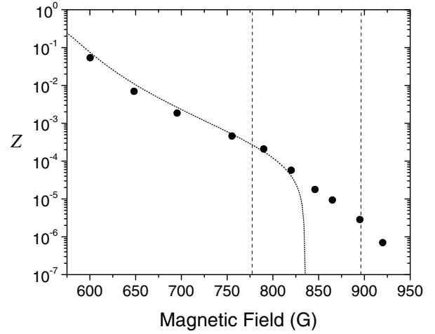
FIG. 4. Z vs B . The closed circles represent the value of Z extracted from measured values of \Gamma . In the case of the 920 G point, the loss is not exponential, but the value of \Gamma is taken to be the initial loss rate. The uncertainty in Z is approximately equal to the size of the closed circles, and is due mainly to uncertainty in the probe laser intensity. The dotted line shows a comparison with results obtained from a coupled channels calculation [15]. The vertical dashed lines represent the boundaries of the strongly interacting regime, k_F|a| > 1 , where k_F is evaluated using typical values of N at the low- and high-field extremes. Although shot-to-shot variations in N are 30%, the average value of N at each field is between 13000 and 90000 due to day to day variations. T_F is between 200 and 600 nK due to differences in N as well as the trap frequencies. For all the data, T < T_c and for the points above 850 G, T < 0.5T_c , where T_c refers to the critical temperature at 695 G. The gas is expected to be adiabatically cooled by the increasing field ramp for fields above 755 G [16].
