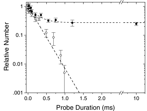
FIG. 2. Loss of signal vs molecular probe duration at 695 G. The open circles correspond to a gas evaporatively cooled to a nearly pure molecular BEC, while the closed circles correspond to full trap depth, where T/T_F \approx 0.75 as measured at 754 G. The dashed lines are fits to exponentials, with a leftover fraction of 25% in the high-temperature case. The time axis for the BEC data was scaled to account for differences in molecular probe laser intensity between the BEC data (30 mW/cm 2 ) and the high-temperature data (15 mW/cm 2 ). We have verified that the loss rate depends linearly on intensity. The error bars represent the statistical standard deviation from the mean of \sim 10 independent measurements.
