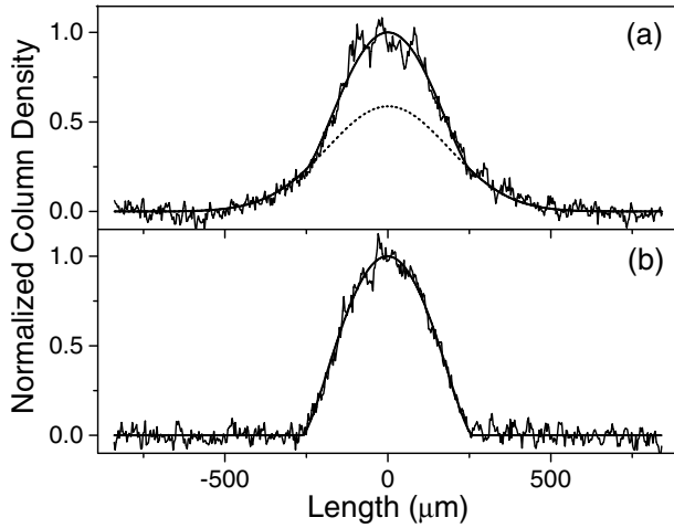
FIG. 1. In-situ absorption image profiles showing a molecular BEC. These images were recorded at a field of 695 G after evaporation at 754 G. For (a), the optical trap depth was lowered to 0.5 \mu\text{K} . The solid line is a fit to a Gaussian (dotted line) plus Thomas-Fermi distribution which distinguishes the condensate from residual thermal molecules. For (b), the trap depth is reduced to 0.27 \mu\text{K} , producing an essentially pure molecular condensate with the number of molecules, N = 46000 . We estimate that the condensate fraction is >90\% , implying T/T_c \leq 0.5 , where T_c is the critical temperature for BEC at 695 G. The solid line is a Thomas-Fermi distribution.
