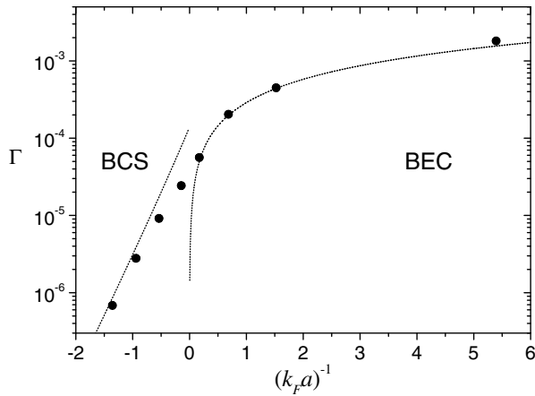
FIG. 5. Comparison of \Gamma with |\Delta|^2 . \Gamma is expressed in units of \Omega^2/\gamma making it equivalent to Z plotted in Fig. 4. The dashed lines correspond to evaluations of |\Delta|^2 in the BCS and the BEC limits integrated over a Thomas-Fermi density profile. They have been scaled by the same factor to give the best fit on the BEC side. |\Delta|^2 is reduced by a factor of 3 on the BEC side to account for an error in Ref. [14].
