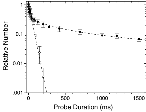
FIG. 3. Same as for Fig. 2, except at 865 G. The dashed line in the case of the full trap depth data (closed circles) is a fit to a “two-fluid” model where one component decays via a rapid one-body loss process and the other via a slower two-body loss process. Approximately 75% of the gas is lost by the initial fast process.
