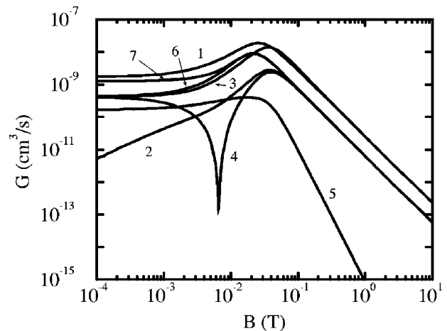
FIG. 2. Exchange decay rate constants for the processes (1) 65→61, (2) 54→63, (3) 54→52, (4) 54→41, (5) 54→21, and (6) 64→62, (7) 64→51 as a function of the magnetic-field strength.
