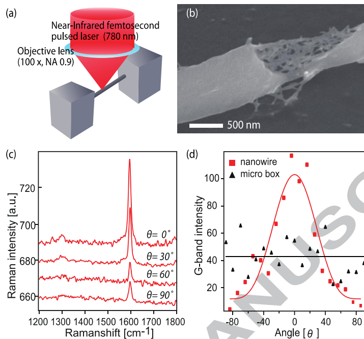
Fig. 4 – (a) A schematic setup for laser ablation. (b) SEM image at a clack produced by laser ablation. (c) Polarized Raman spectra of a 460-nm-wide-nanowire taken at different angles \theta between polarization of the incident laser light and the nanowire axis. Excitation wavelength, laser power and exposure time are 785 nm, 0.6 mW and 10 s, respectively. (d) The angular dependence of G-band intensity. The square and triangle dots are experimental results for the nanowire and the box, respectively. The line is a \cos^4 \theta fitting curve for the nanowire [47].
