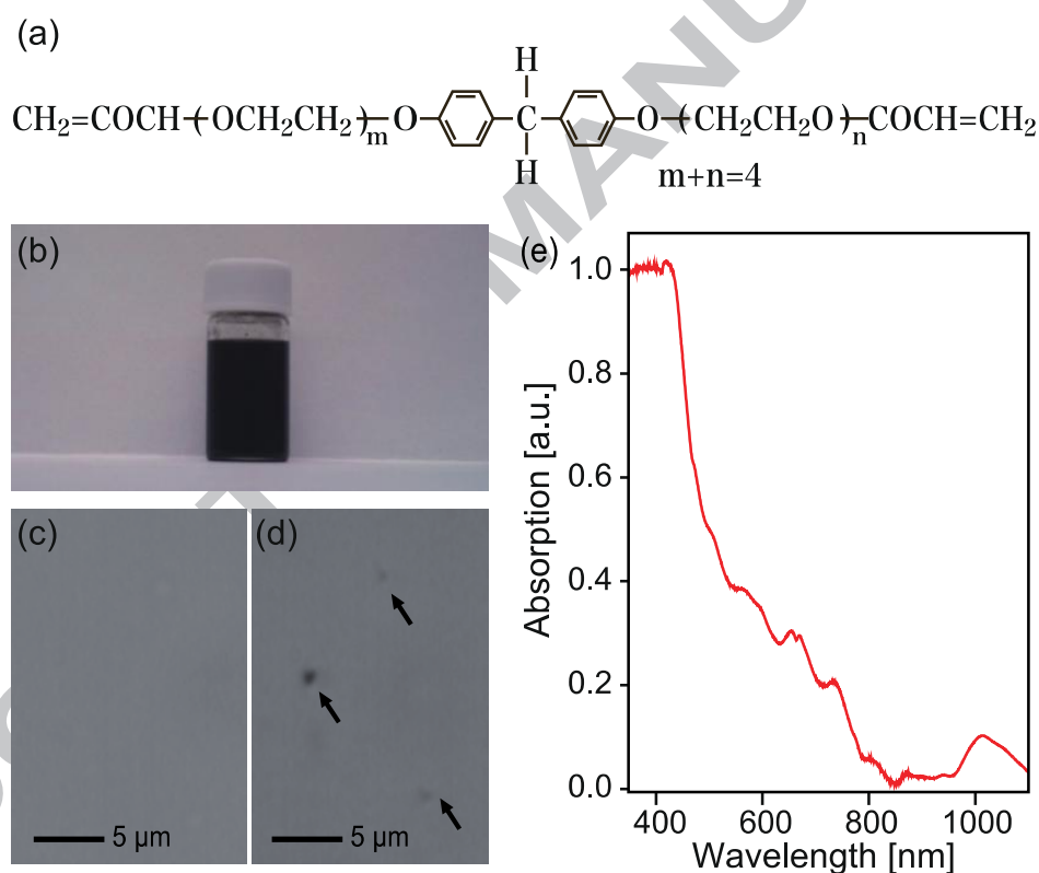
Fig. 1 – (a) The chemical structure of R712. (b) A photograph of the SWCNT-dispersed resin. (c) A bright field image of the SWCNT-dispersed resin. (d) A bright field image of the SWCNT-dispersed resin after 3 h from sonication. (e) An absorption spectrum of the SWCNT-dispersed resin.
