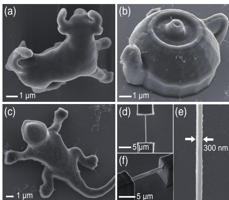
Fig. 2 - 3D micro/nano structural SWCNT/polymer composites are fabricated by using the TPP lithography. The structures in (a)-(f) are a 8- \mu\text{m} -long micro bull, a micro tea pod, a micro lizard, a nanowire suspended between two micro boxes, magnified image of (d), and perspective view of the nanowire, respectively.
