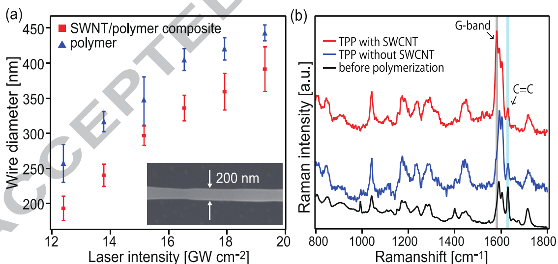
Fig. 5 – (a) The spatial resolution, which is estimated from wire width, as a function of laser intensity. Wire widths of SWCNT/polymer composites and those of polymer are indicated by the square and the triangle, respectively. (Inset) SEM image of a
