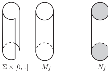
Fig. 1. M_f and N_f .
