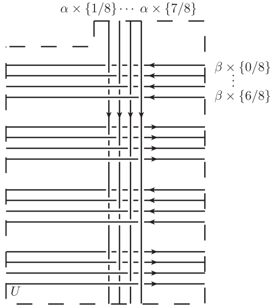
Fig. 7. Attaching curves when N = 3 .
