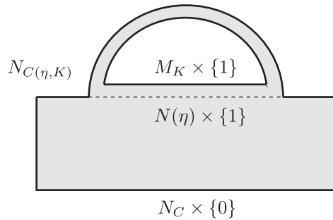
Fig. 9. The 4-manifold W with \partial W = N_C \sqcup -N_{C(\eta,K)} \sqcup M_K .
