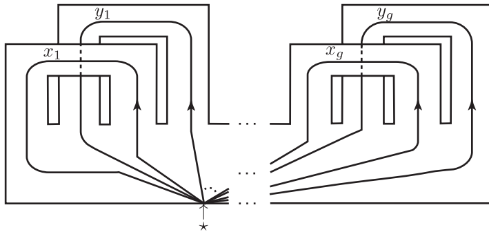
Fig. 4. The curves x_i and y_i generate the fundamental group of the punctured surface \Sigma_{g,1} .
