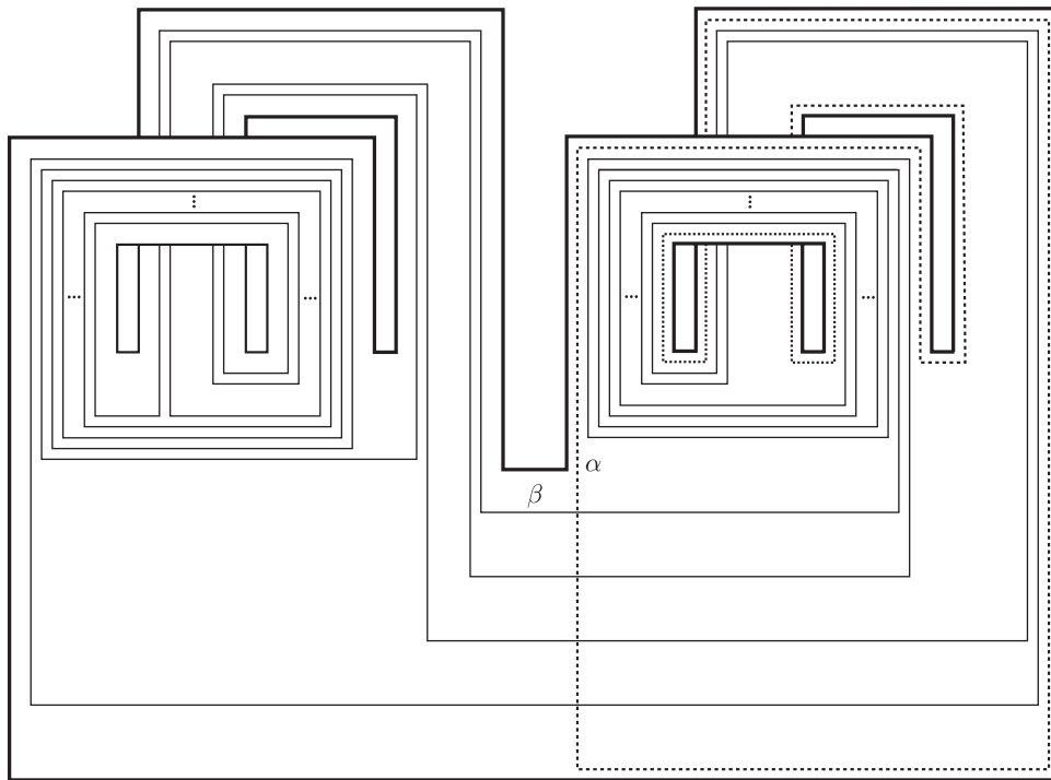
Fig. 5. The curves \alpha and \beta .
