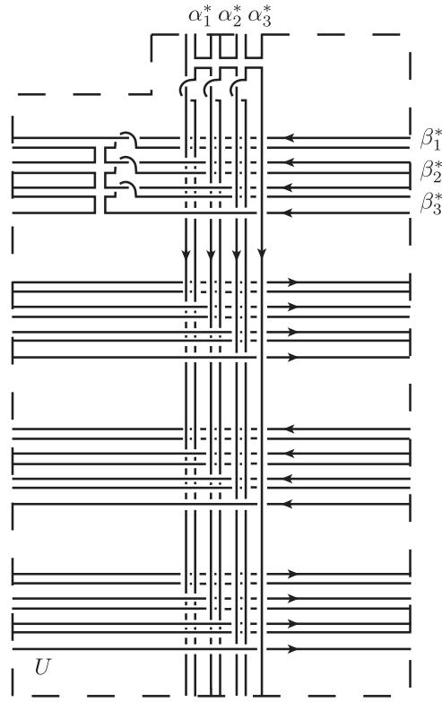
Fig. 8. Attaching curves after handle slides when N = 3 .
