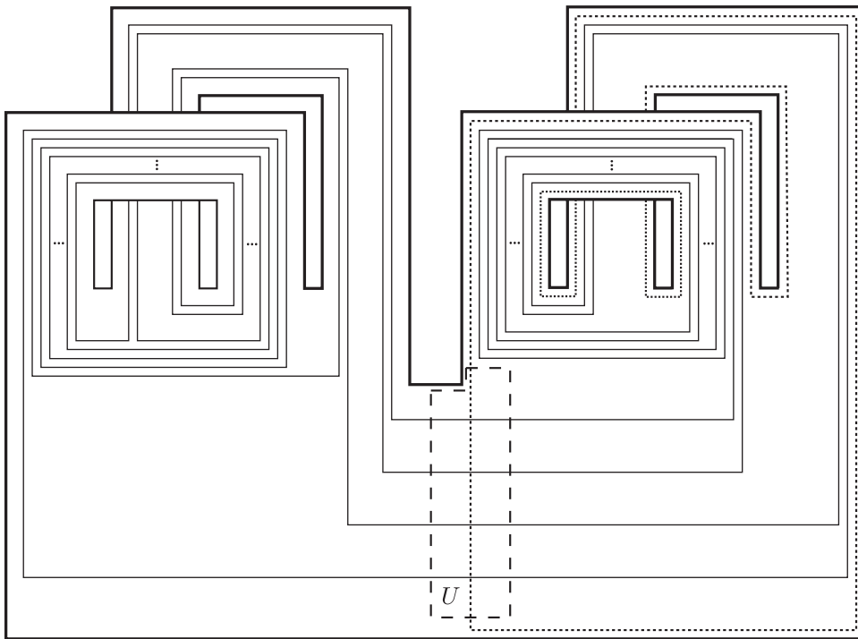
Fig. 6. The region U in \Sigma .
