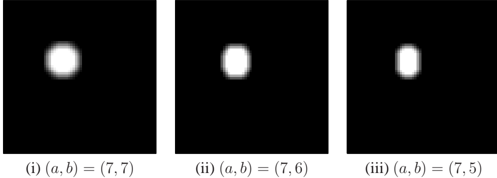
Figure 3: Three articulation manifolds embedded in \mathbb{R}^{4096} sharing a common 2-D parameter space \Theta .
