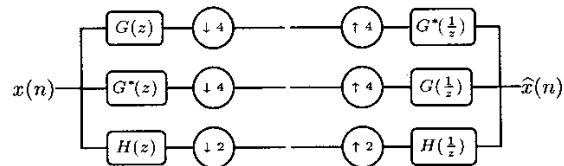
Fig. 1. Orthoconjugate filter bank structure.
