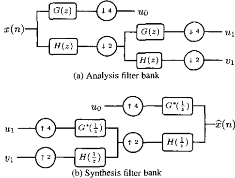
Fig. 2. Analysis and synthesis filter banks with real input signal x(n) . The band filtered by G^* in Fig. 1 can be eliminated.
