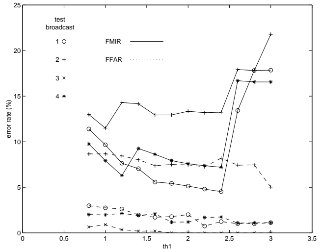
Figure 2. Frame based error rates as a function of th1 using target model Brokaw1 and background models Back3 and BackComm1
