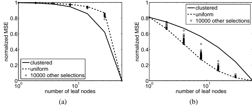
FIG 5. Comparison of probing schemes for a WIG model with (a) negative correlation progression and (b) positive correlation progression. Observe that the clustered nodes are optimal in (a) while the uniform is optimal in (b). The uniform and the clustered leaf sets give the worst performance in (a) and (b) respectively, as expected from our theoretical results.
