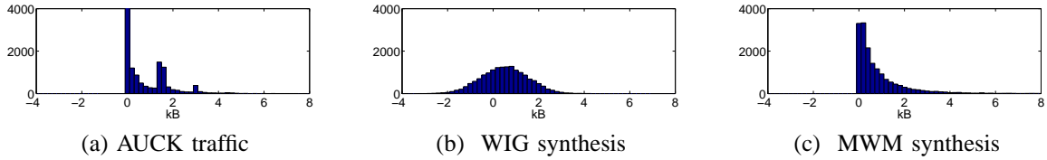
Fig. 4. Histograms of the bytes-per-time processes at time-scale 2ms for (a) wide-area traffic at the University of Auckland (trace AUCK) [22], (b) one realization of the WIG model, and (c) one realization of the MWM.
