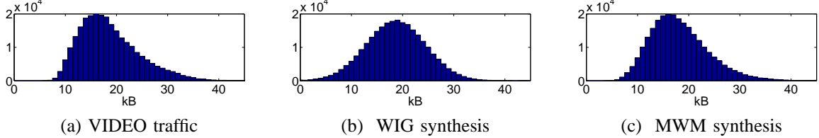
Fig. 5. Histograms of the bytes-per-time processes at time-scale 2.77ms for (a) video traffic formed by multiplexing 15 video traces (trace VIDEO), (b) one realization of the WIG model, and (c) one realization of the MWM. Note that the MWM matches the marginal of the video traffic better than the WIG; however, the video traffic is more Gaussian than the AUCK traffic.
