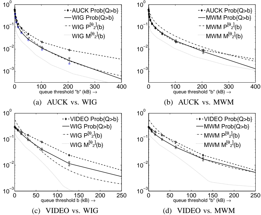
Fig. 6. Queuing performance of real data traces and synthetic WIG and MWM traces at high utilization. In (b), we observe that the MWM synthesis matches the queuing behavior of the AUCK data closely, while in (a) the WIG synthesis is not as close. In (c) and (d), we observe that both the WIG and the MWM match the queuing behavior of VIDEO. We also observe that the product approximation ( P^{[\theta_2]}(b) ) is close to the empirical queuing behavior for both synthetic traffic loads (both WIG and MWM) and that it performs better than the max approximation, M^{[\theta_2]}(b) .
