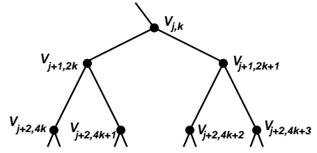
Fig. 1. Multiscale tree representation of a traffic trace. Nodes at each horizontal level in the tree correspond to the sum (aggregates) of the process in non-overlapping blocks of sizes of powers of two, with lower levels corresponding to smaller block sizes. Each node is the sum of its two child nodes.
