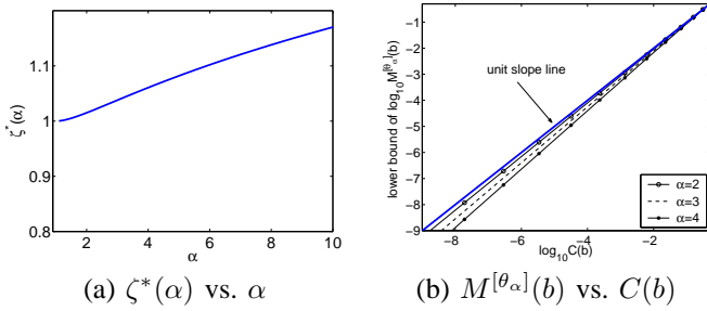
Fig. 2. (a) For a large range of \alpha , \zeta^*(\alpha) is close to 1. (b) Observe that the lower bound of M^{[\theta_\alpha]}(b) is almost identical to the upper bound C(b) .
