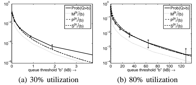
Fig. 3. Comparison of the max, the product and the sum approximations to \mathbb{P}\{Q > b\} for fGn traffic with parameters H = 0.8 , link capacity 10Mbps and \sigma = 8 \times 10^5 bits. For different utilizations in (a) and (b), the product and sum approximations are close to \mathbb{P}\{Q > b\} for a wide range of queue thresholds b . The max approximation is a lower bound of \mathbb{P}\{Q > b\} and is accurate to an order of magnitude.
