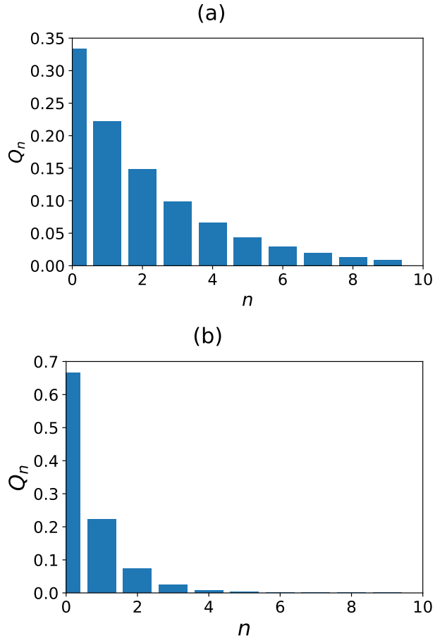
Figure 3: The probability to divide Q_n as a function of cell size n for: (a) \lambda/k = 2 (b) \lambda/k = 0.5 .
