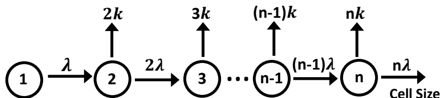
Figure 1: A schematic view of a discrete-state stochastic model of the cell-size regulation. The cell size is described by a discrete variable n that corresponds to the number of proteins responsible for growth.
