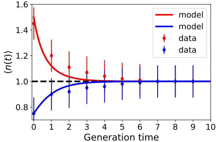
Figure 2: The normalized cell length as a function of the time in units of inter-division generation time. Solid lines are theoretical predictions from Eq. (3) and symbols are from experimental observations for E.coli bacteria as given in Ref. 2
