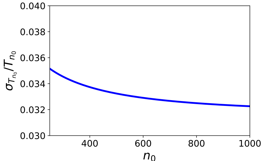
Figure 6: The normalized variance of inter-division times as a function of the initial cell size n_0 . The calculations are done using the same parameters as in Fig. 5
