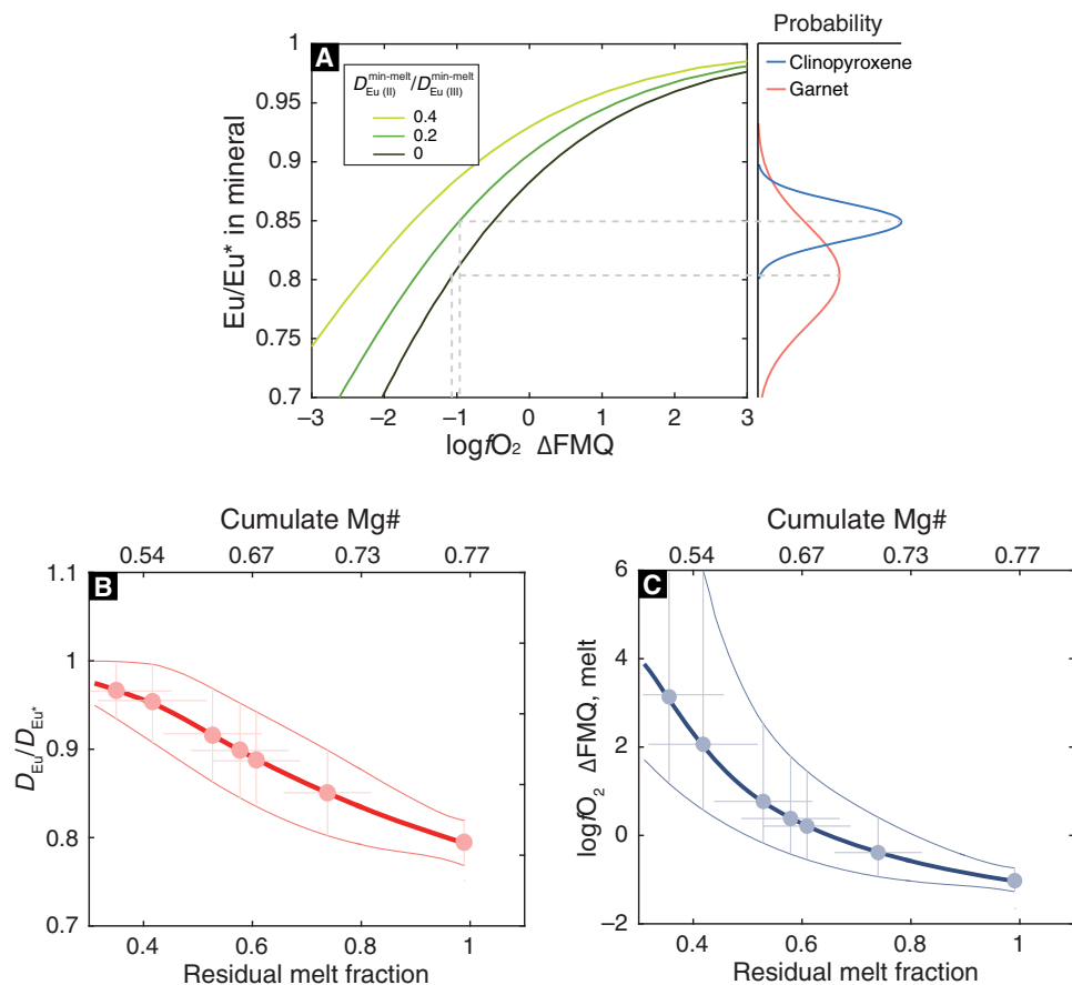
Fig. 2. Magma redox conditions calculated from garnet and clinopyroxene Eu anomalies. (A) Estimating fO_2 of primitive magma. Garnet and clinopyroxene Eu/Eu^* - fO_2 plotted on the contours of D_{Eu(II)}^{min-melt}/D_{Eu(III)}^{min-melt} . The probability distribution is for sample CC-ME1, the second most primitive garnet-bearing pyroxenite in this work. (B) Evolution of the bulk Eu partition coefficient relative to D_{Eu^*} (bulk partition coefficient of Eu^{3+} ) during crystal fractionation, calculated using the observed Eu/Eu^* of garnets and an incremental crystal fractionation model (see the Supplementary Materials and Methods). Dots with error bars (95% confidence interval) represent D_{Eu}/D_{Eu^*} values estimated from Eu/Eu^* of garnets in cumulates. Residual melt fraction estimated by converting whole-rock cumulate Mg# to the Mg# of a melt in equilibrium with the cumulate and inferring melt fraction from empirical relationships between melt Mg# and indices of melt fraction, such as K_2O (see the Supplementary Materials and Methods). The uncertainties are from the measured garnet Eu/Eu^* and cumulate-melt Mg# coupling and are propagated into the calculated D_{Eu}/D_{Eu^*} and fO_2 by a Monte Carlo resampling method (see the Supplementary Materials and Methods). Thick red line demarcates median values, and thin red line displays 95% confidence interval envelope. The total Eu partition coefficients in (B) were converted to fO_2 in (C). Clinopyroxenes show the same Eu/Eu^* -Mg# trend as garnet (Fig. 1), but we use garnet data to calculate the redox paths because the perfect incompatibility of Eu^{2+} in garnet simplifies Eq. 1 and reduces uncertainty.
