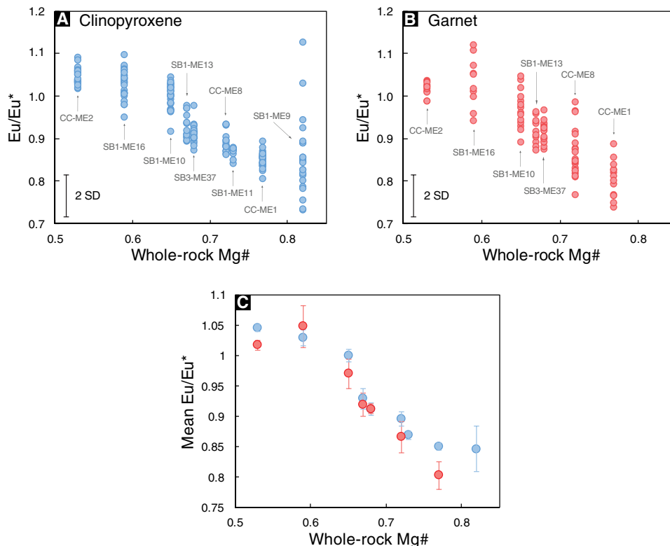
Fig. 1. Eu/Eu* in clinopyroxene and garnet in deep arc cumulates as a function of whole-rock Mg#. (A and B) Individual spot data measured by laser ablation ICP-MS. The error bars denoted in (A) and (B) are the long-term (~8 months) reproducibilities (2 SD) of measuring Eu/Eu* in basaltic glass standards BIR-1G and BCR-2G. (C) The mean Eu/Eu* in clinopyroxene and garnet for each rock sample. Error bars are 2 standard error of mean (2 SEM).
