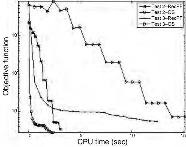
Fig. 3. Comparing RecPF with OS: objective value versus CPU time.
