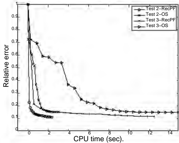
Fig. 4. Comparing RecPF with OS: relative error versus CPU time.
