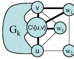
Figure 3.1: The augmented graph \tilde{G}_k .
