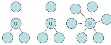
Figure 4.1: Three examples of 2-claws.
