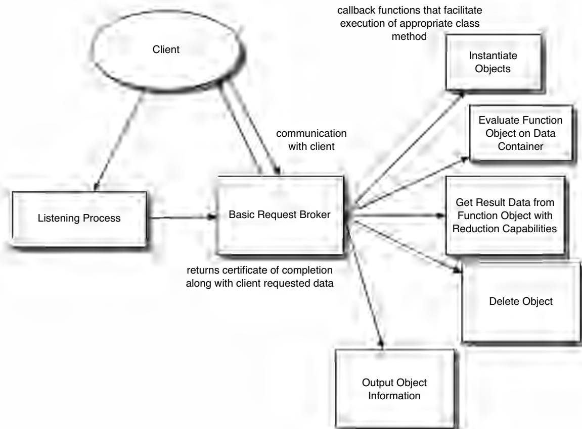
Figure 2.2 Server Behavior
