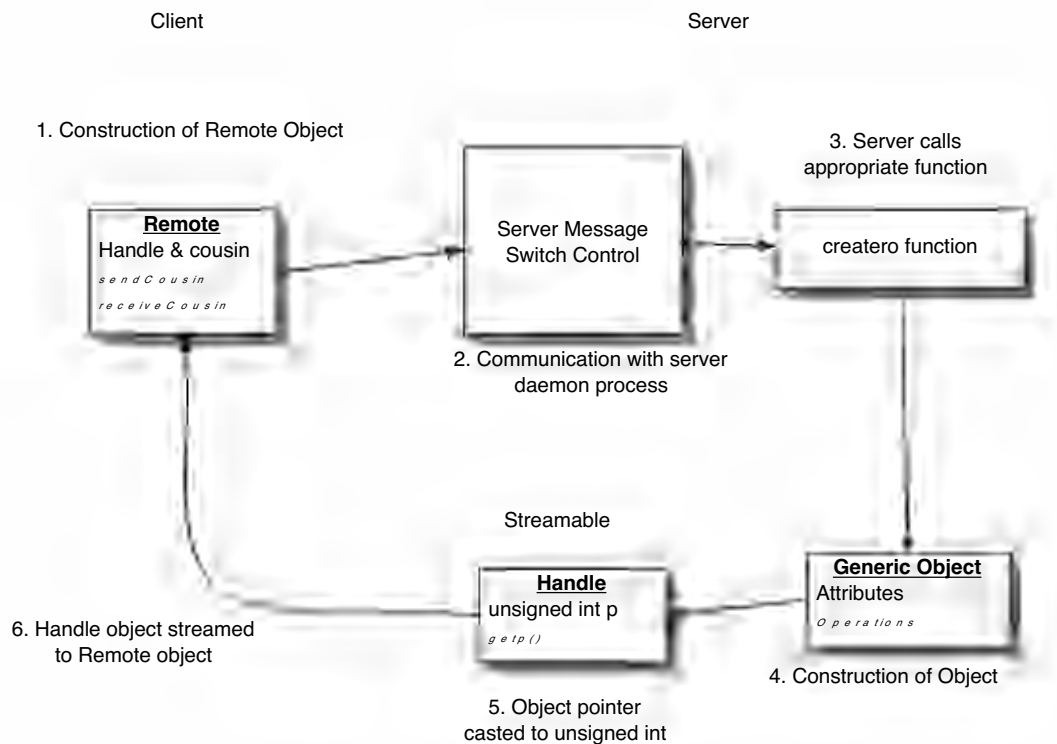
Figure 4.3 Distributed Object Construction
