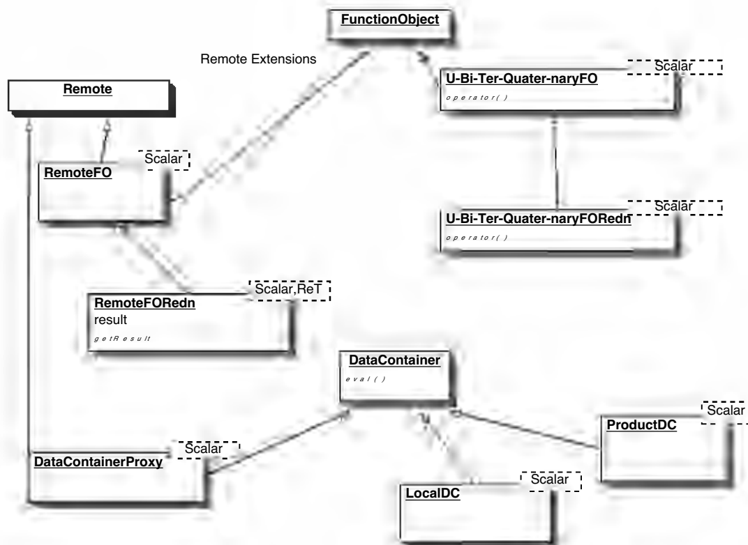
Figure 2.3 Base Class Remote Design: The Remote and Proxy classes (left) make use of double inheritance to extend the base classes (right).
