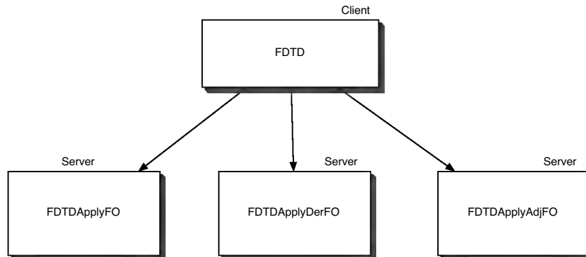
Figure 2.7 Strategy Design in FDTD
