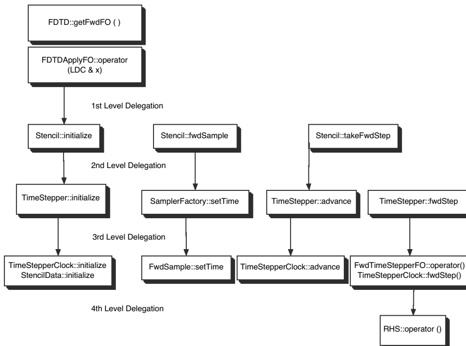
Figure 5.1 Delegation in Euler FDTD
