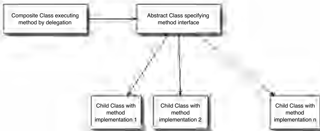
Figure 2.4 Strategy Design Pattern
