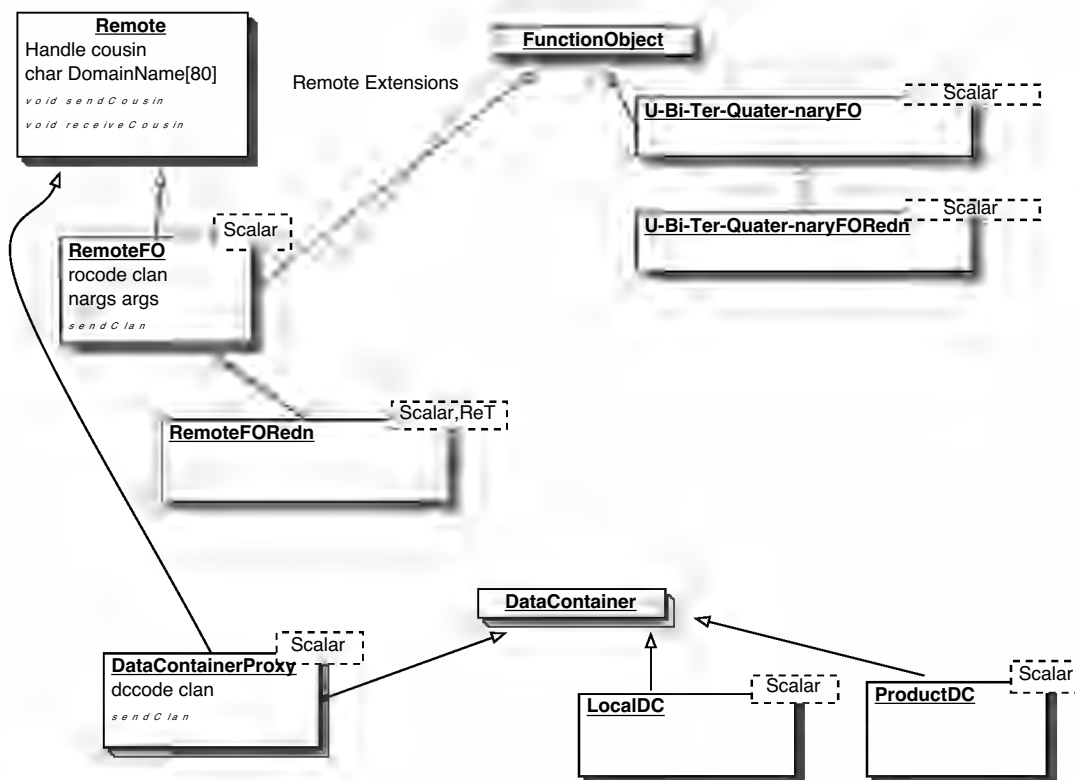
Figure 4.1 Base Class Remote Implementation
